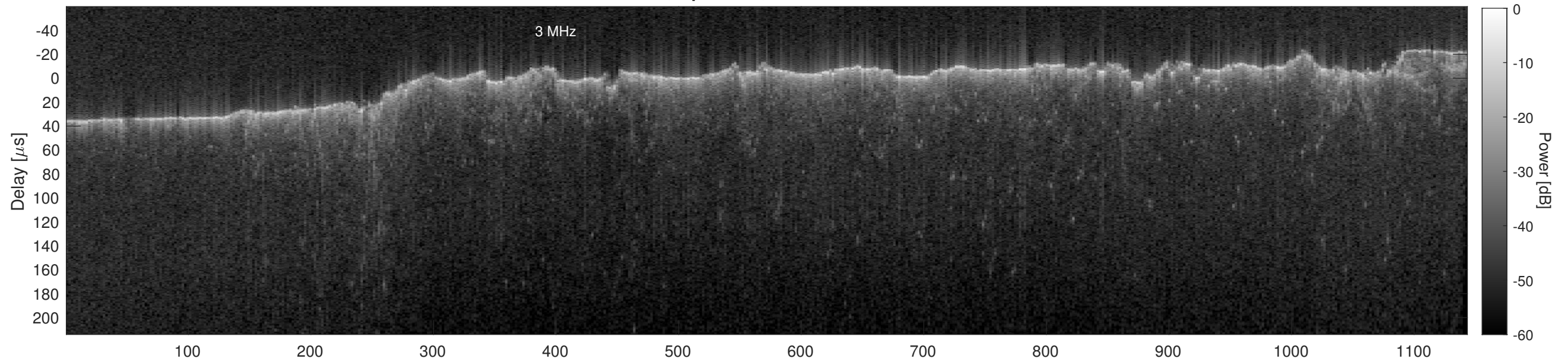
Orbit 17486, Cluttergram
