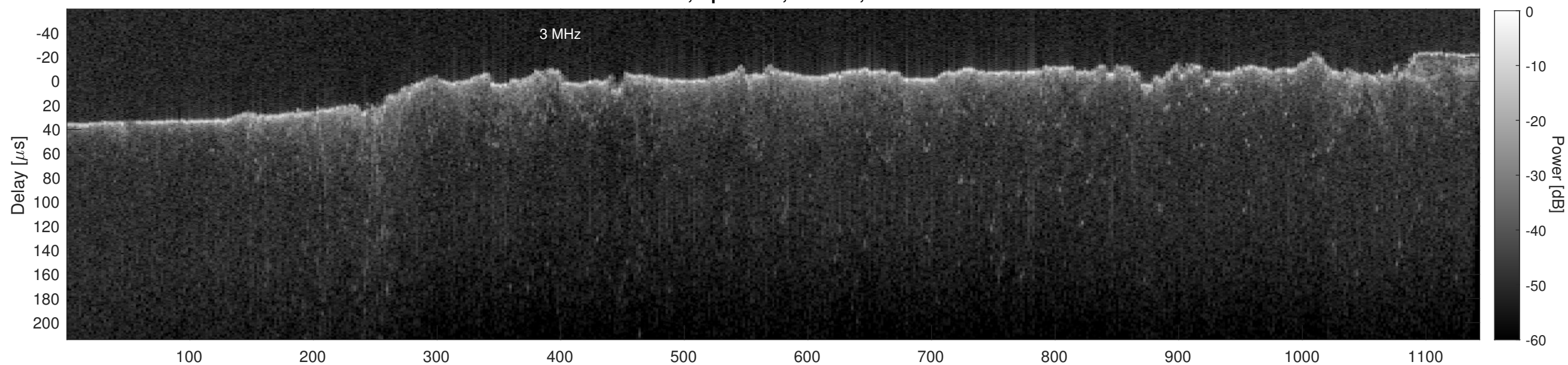
Orbit 17486, Cluttergram
