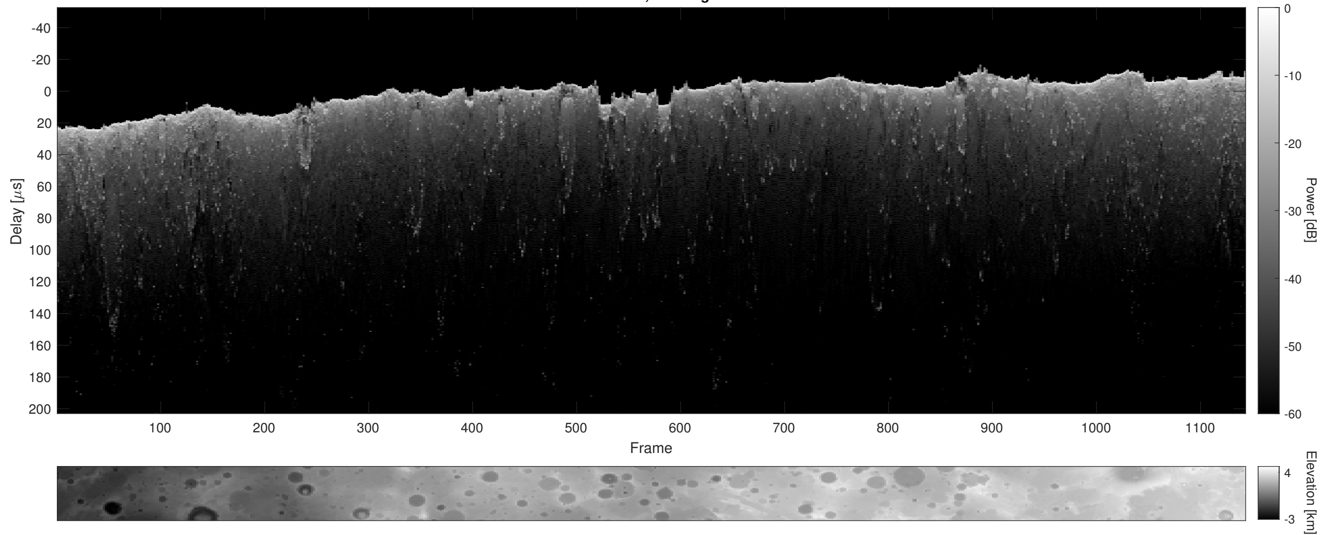
Orbit 17487, Cluttergram
