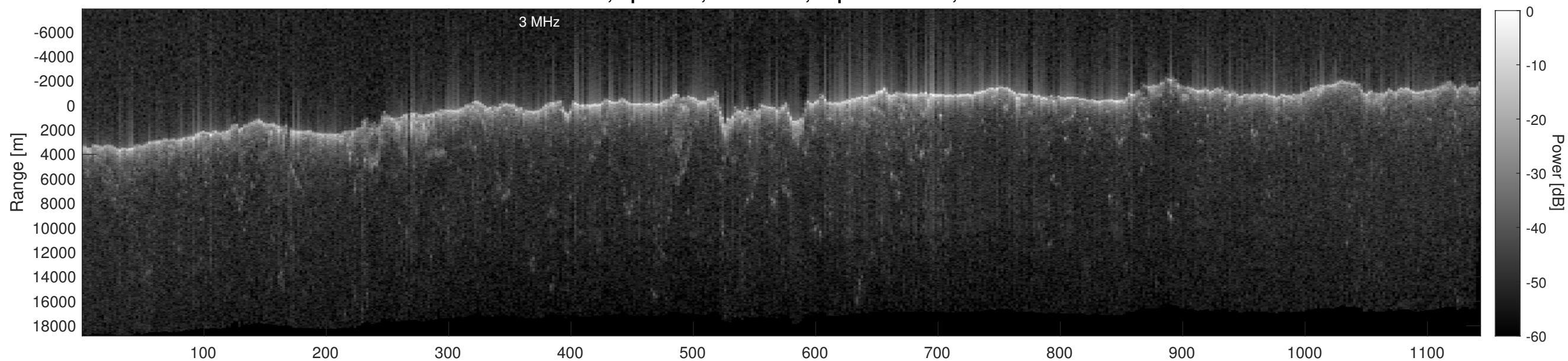
Orbit 17487, Depth-Corrected Cluttergram
