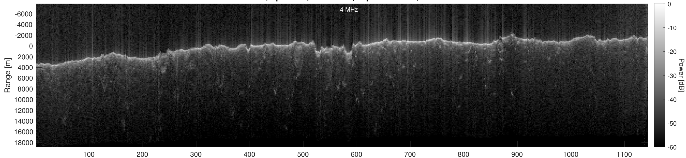
Orbit 17487, Optimized, No Window, Depth-Corrected, Channel 2
