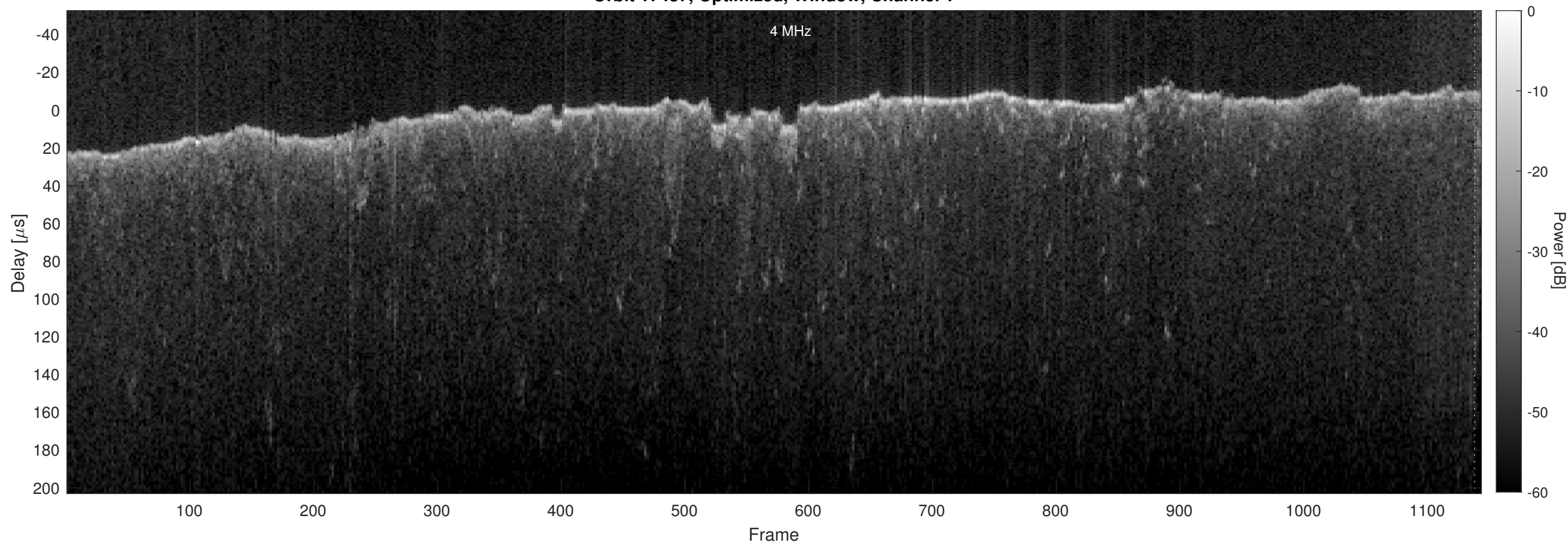
Orbit 17487, Optimized, Window, Channel 2
