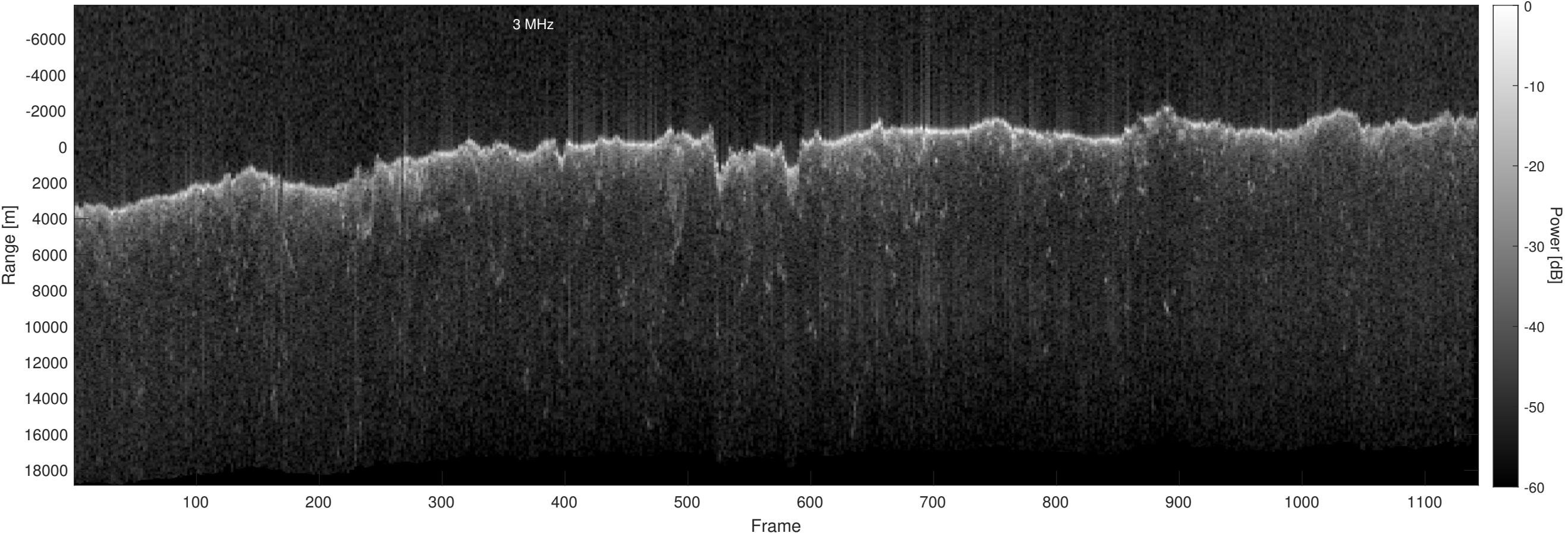
Orbit 17487, Optimized, Window, Depth-Corrected, Channel 2
