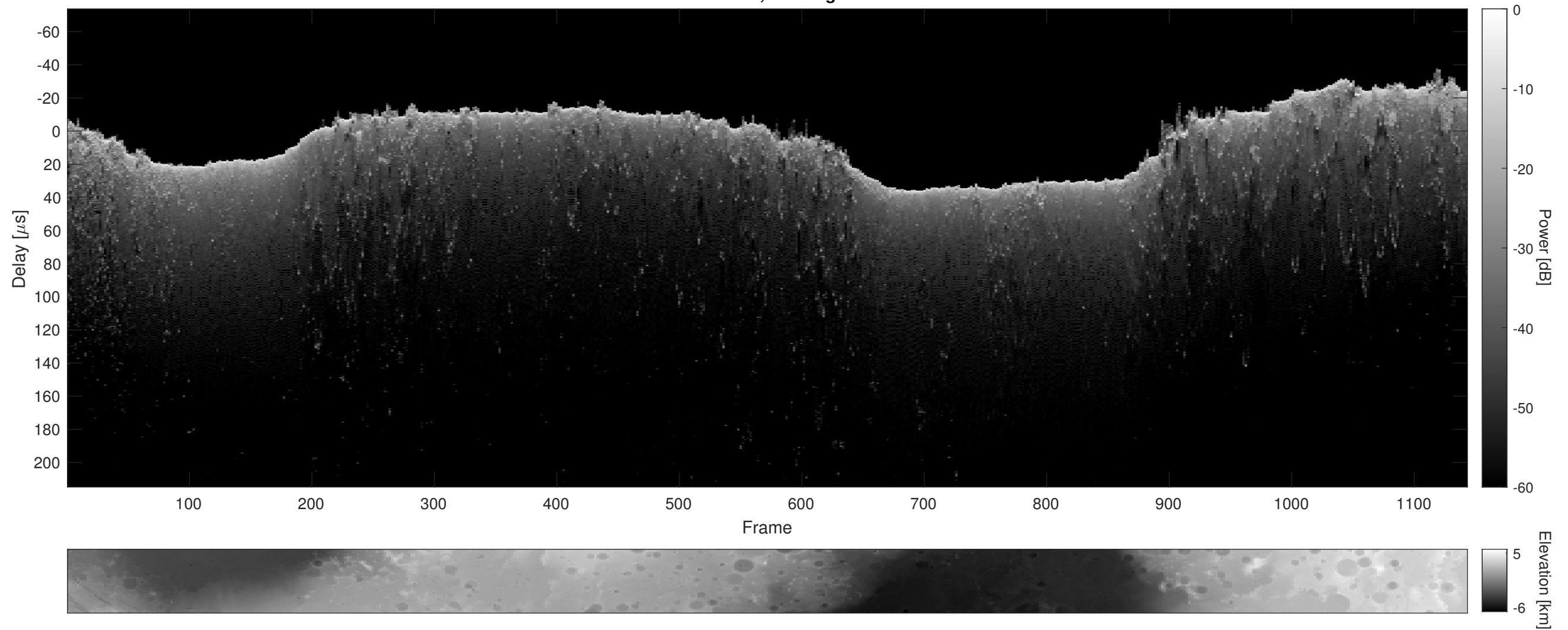
Orbit 17490, Cluttergram
