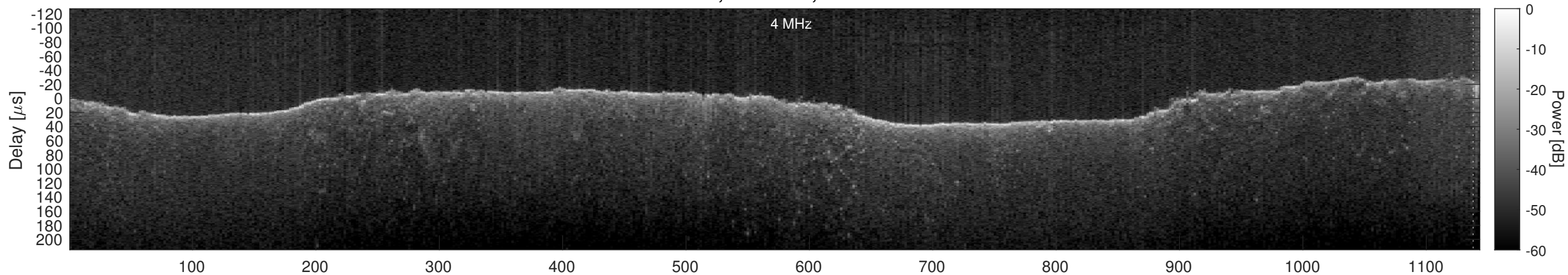
Orbit 17490, Window, Channel 1, Chapman
