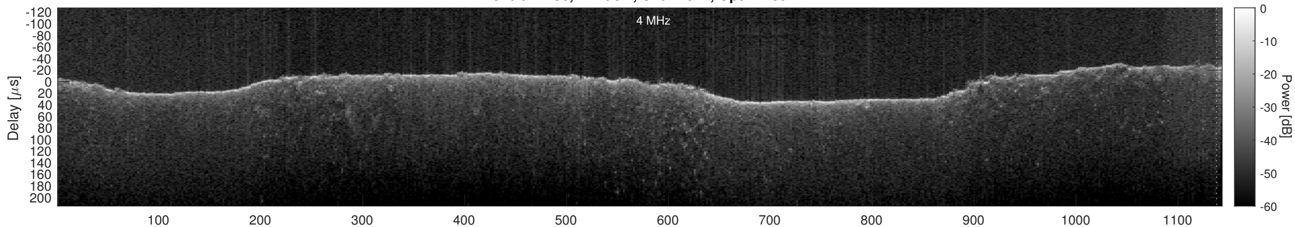
Orbit 17490, Cluttergram
