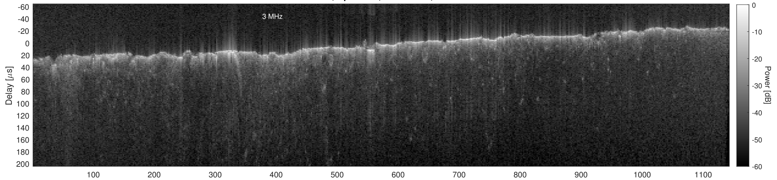
Orbit 17491, Cluttergram
