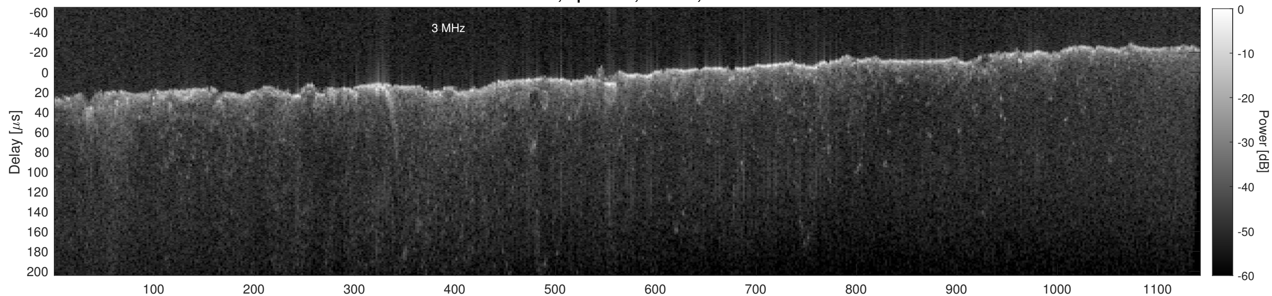
Orbit 17491, Cluttergram
