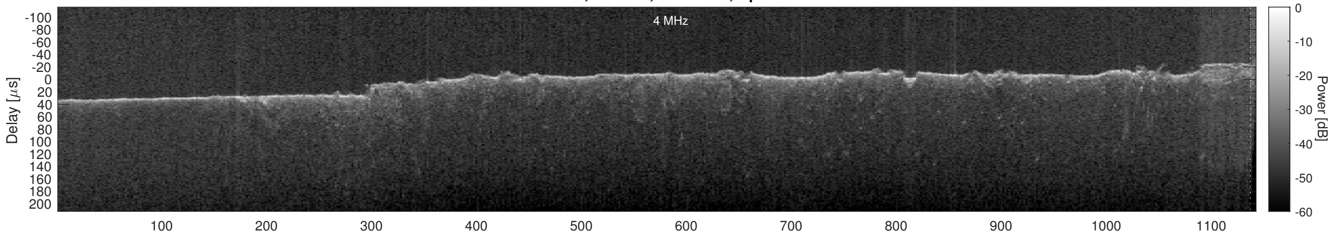
Orbit 17493, Cluttergram
