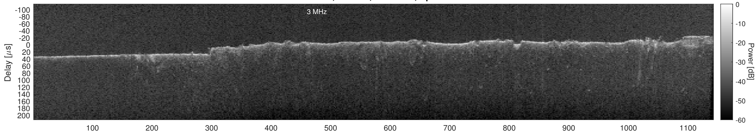
Orbit 17493, Cluttergram
