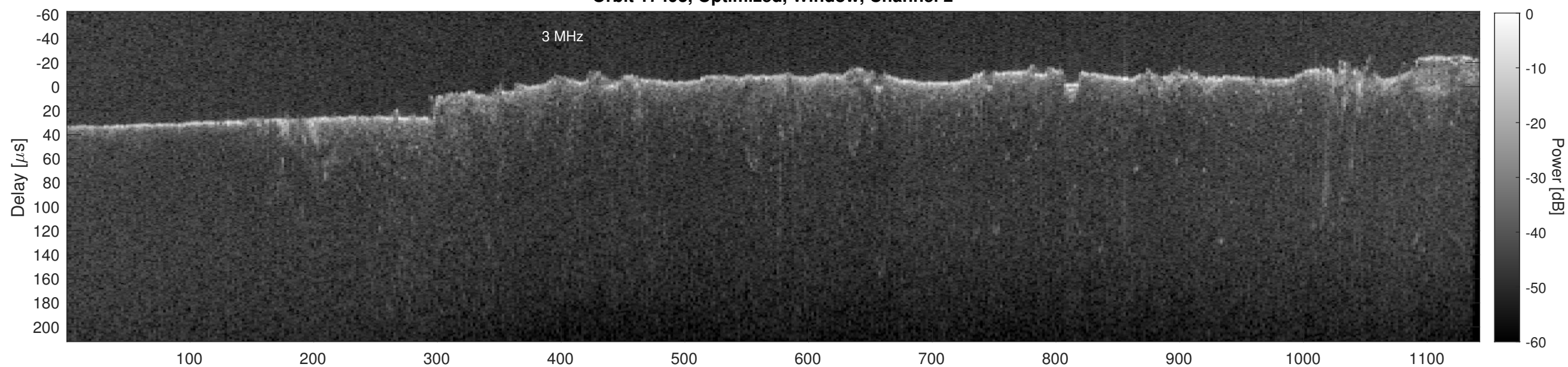
Orbit 17493, Cluttergram
