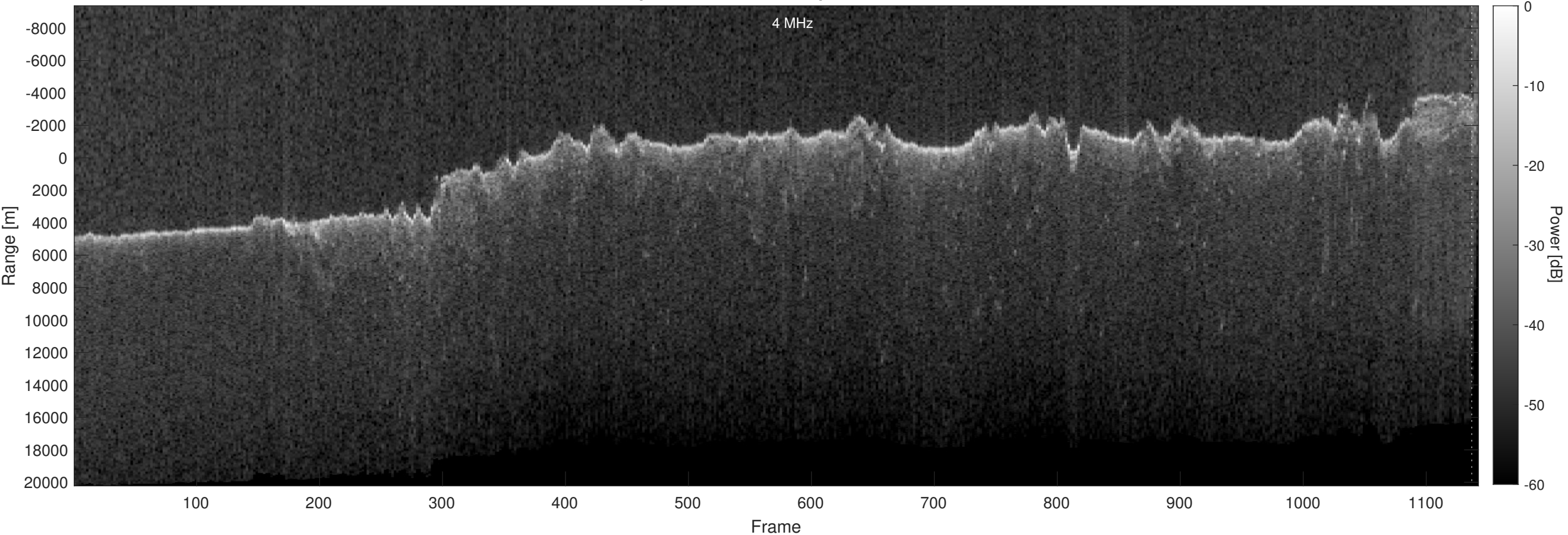
Orbit 17493, Optimized, Window, Depth-Corrected, Channel 2
