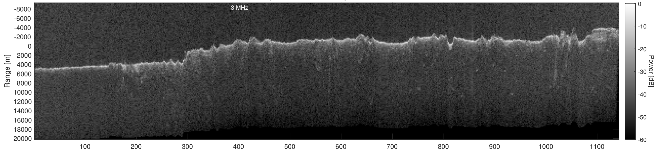
Orbit 17493, Depth-Corrected Cluttergram
