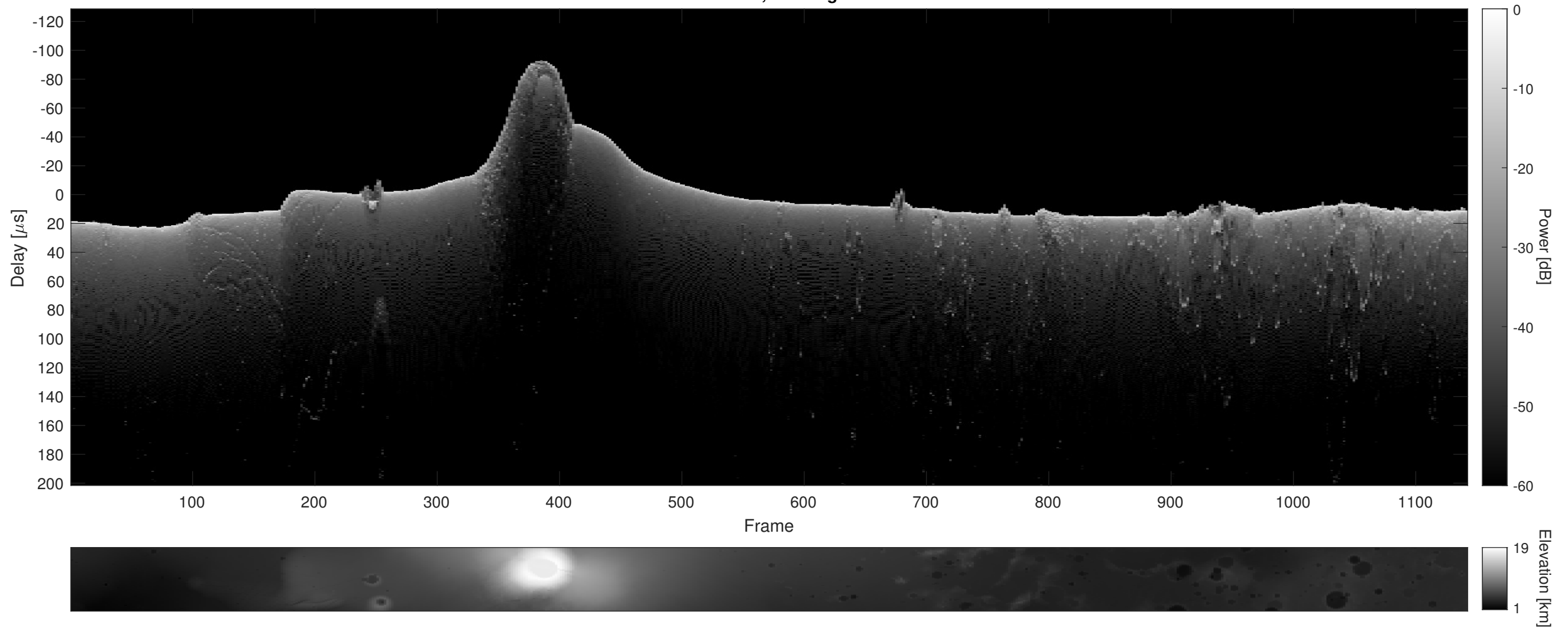
Orbit 17499, Cluttergram
