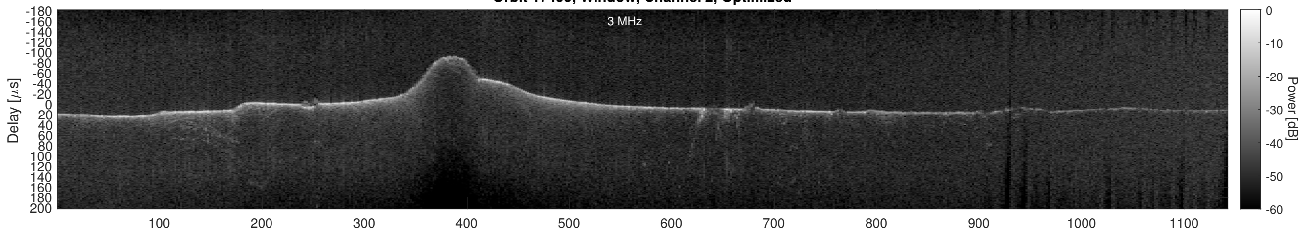
Orbit 17499, Cluttergram
