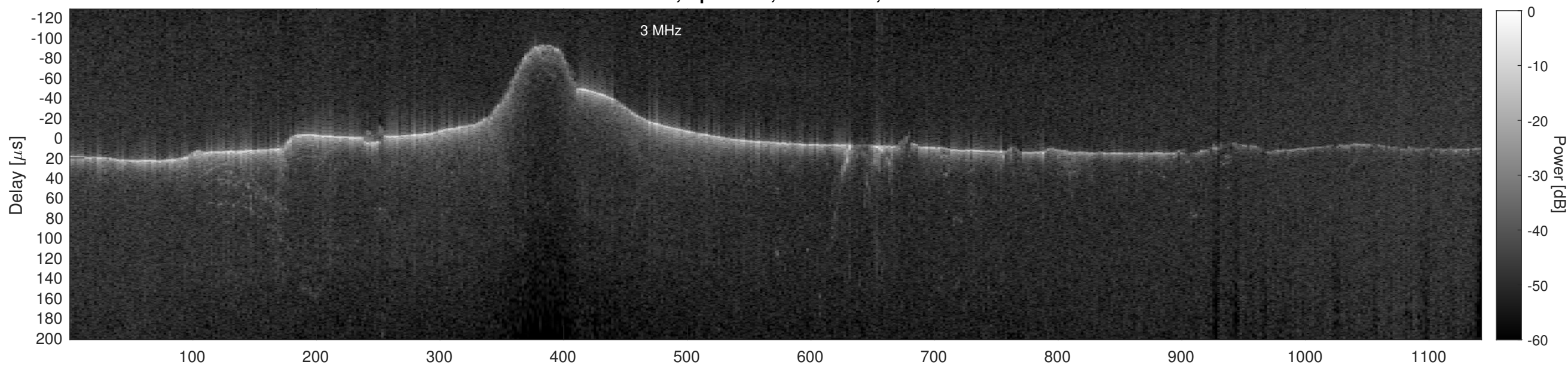
Orbit 17499, Cluttergram
