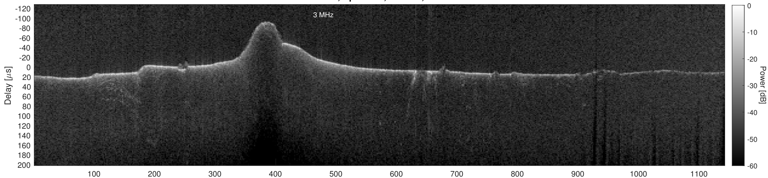
Orbit 17499, Cluttergram
