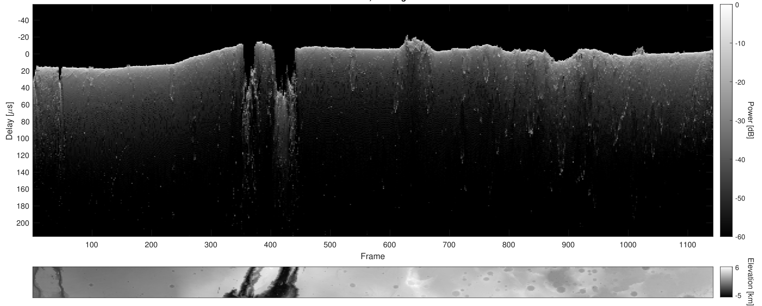
Orbit 17502, Cluttergram
