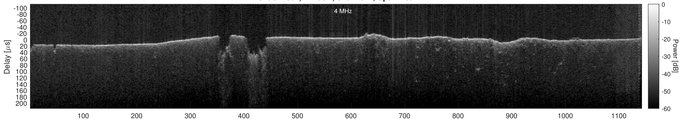
Orbit 17502, Cluttergram
