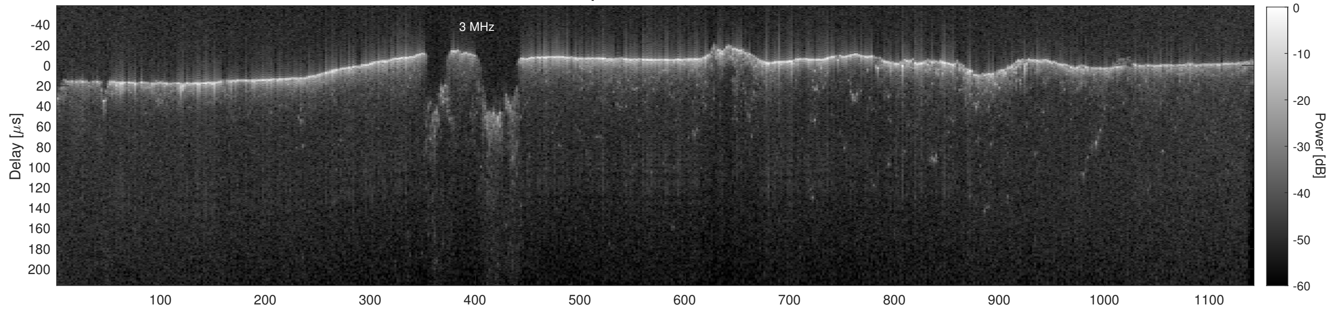
Orbit 17502, Cluttergram
