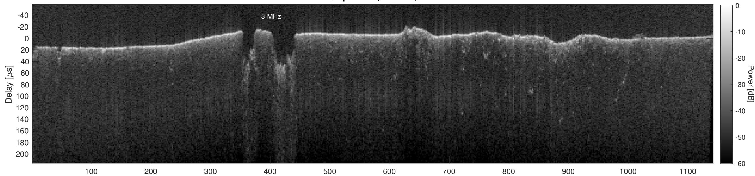
Orbit 17502, Cluttergram
