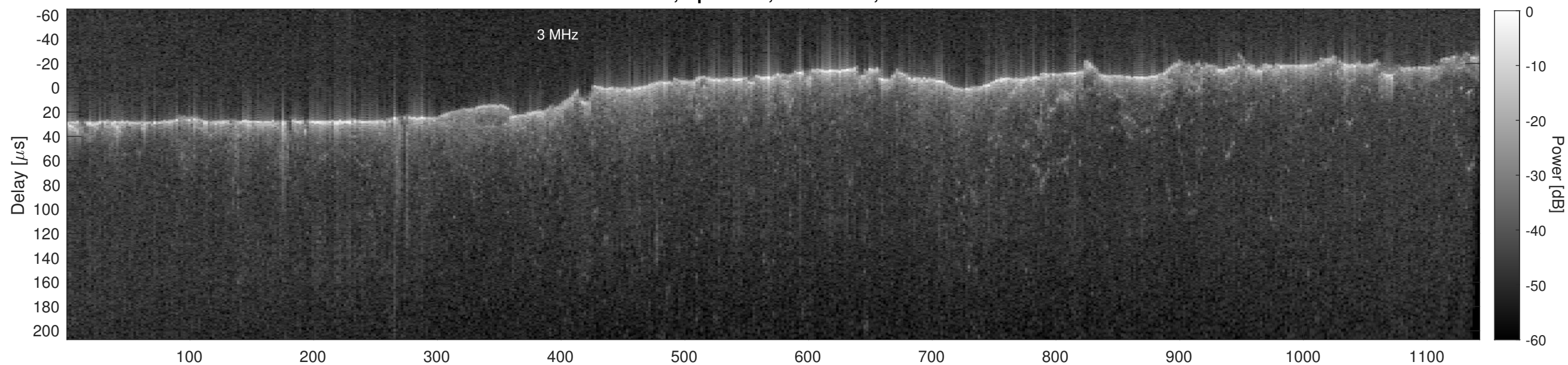
Orbit 17503, Cluttergram
