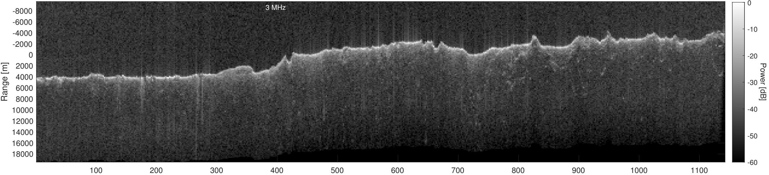
Orbit 17503, Depth-Corrected Cluttergram
