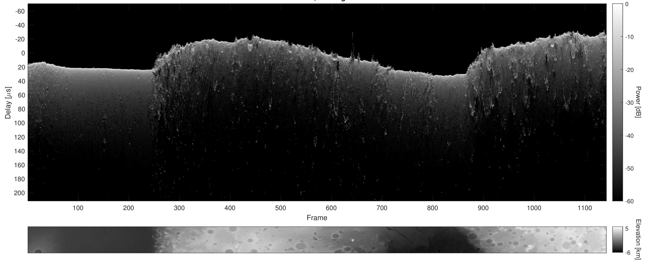
Orbit 17504, Cluttergram
