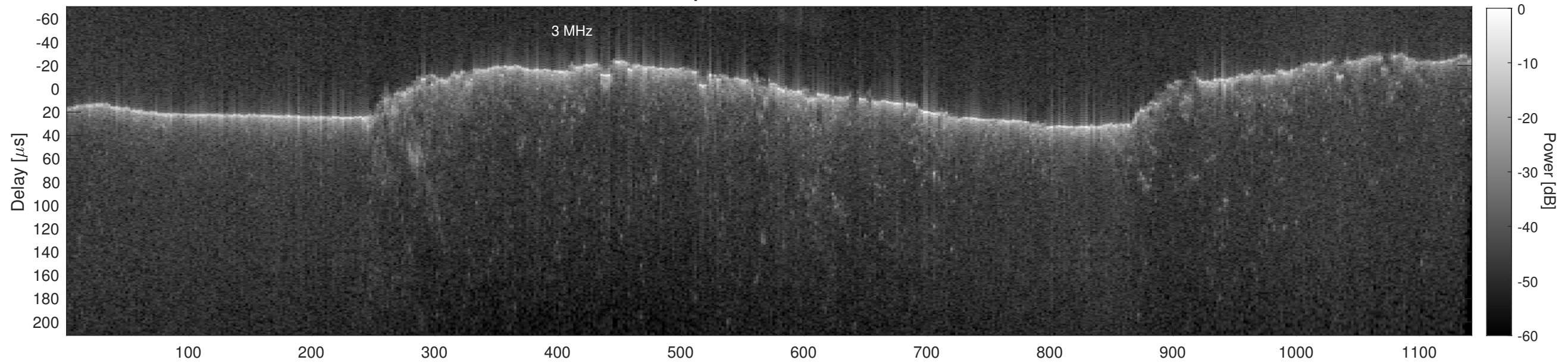
Orbit 17504, Cluttergram
