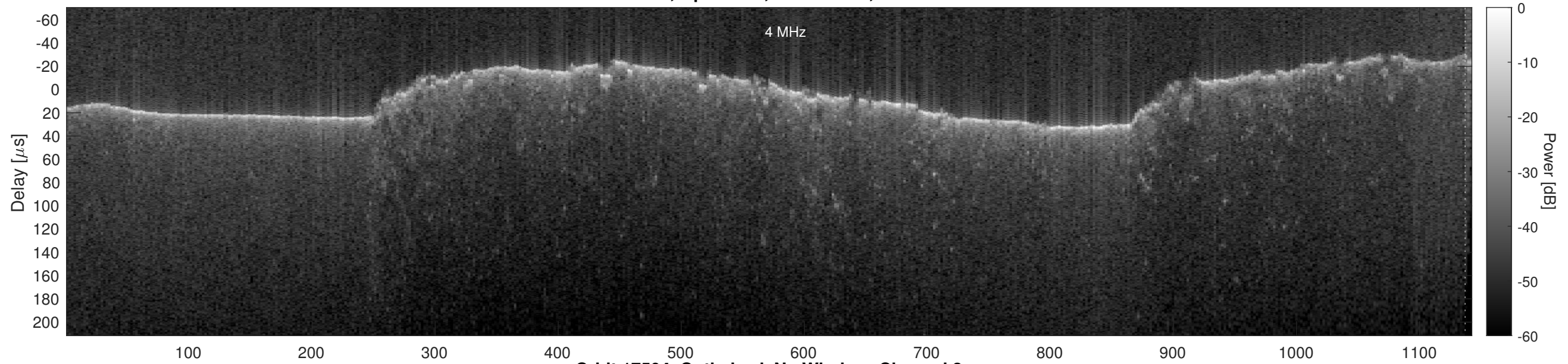
Orbit 17504, Optimized, No Window, Channel 2
