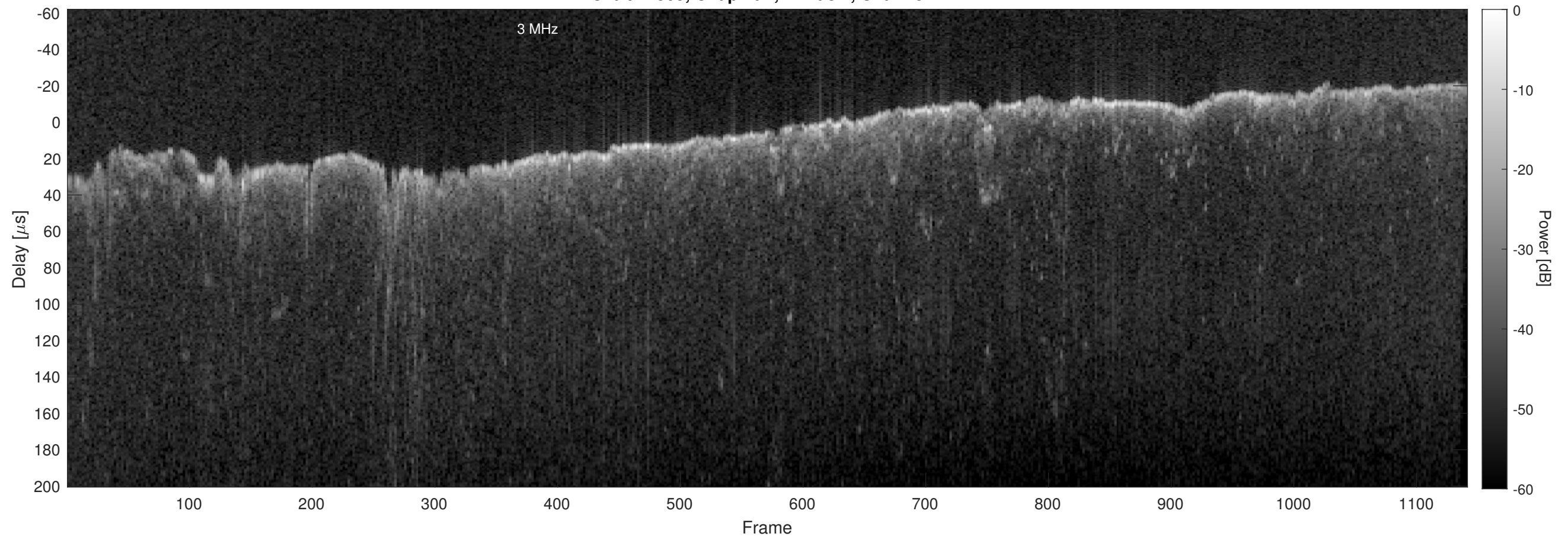
Orbit 17505, Chapman, Window, Channel 2
