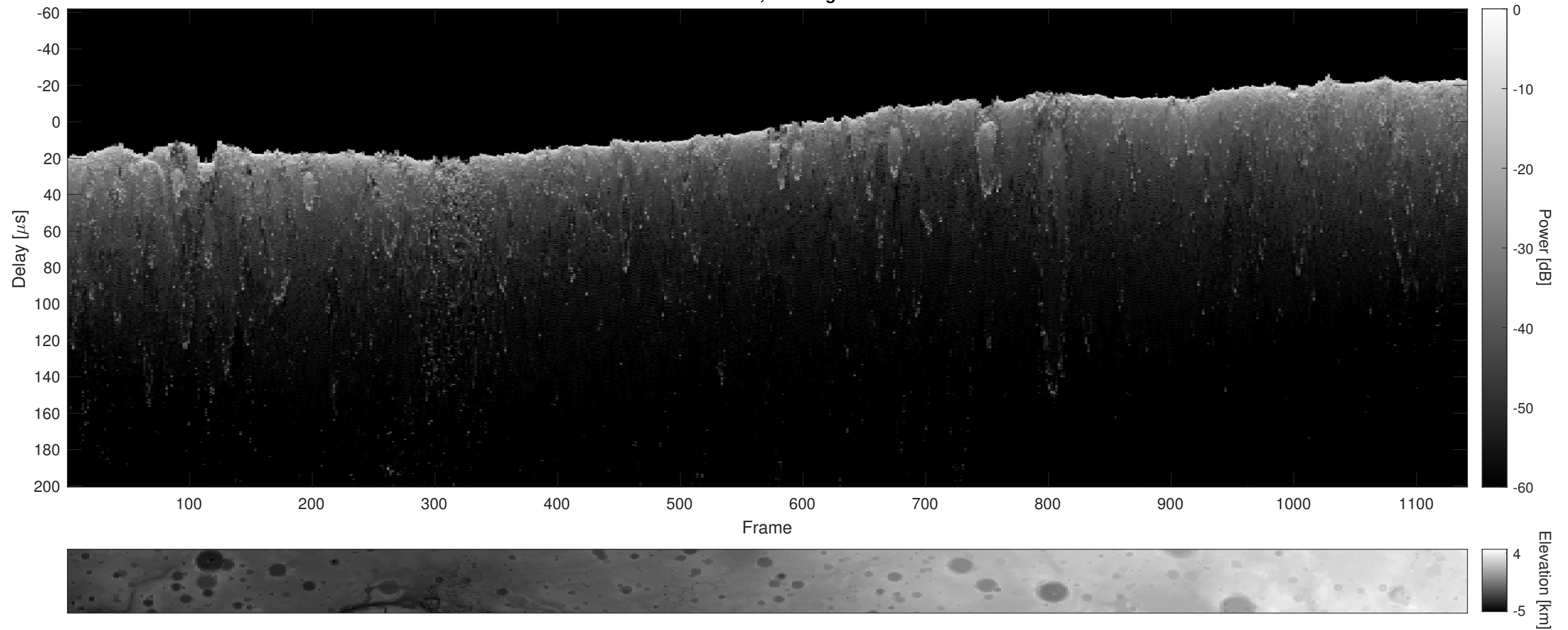
Orbit 17505, Cluttergram
