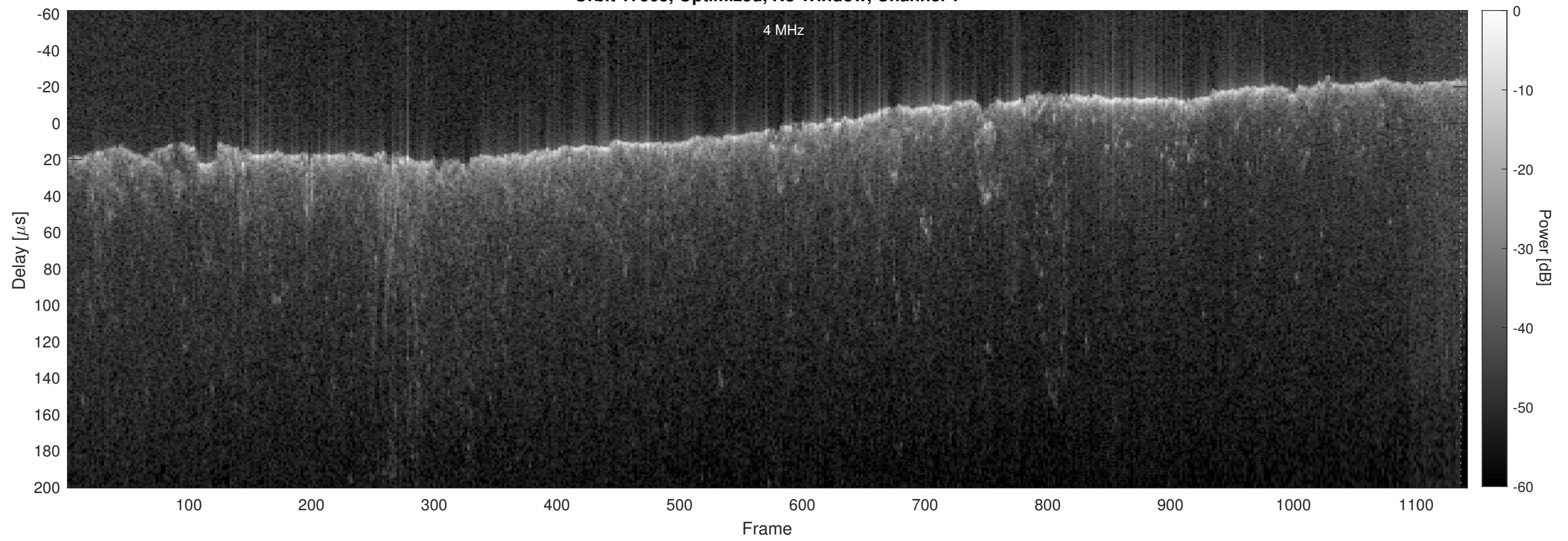
Orbit 17505, Optimized, No Window, Channel 2
