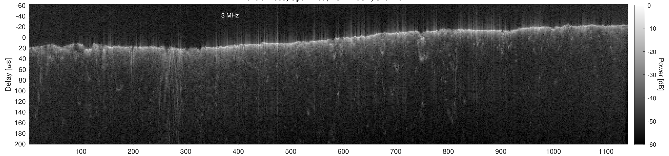
Orbit 17505, Cluttergram
