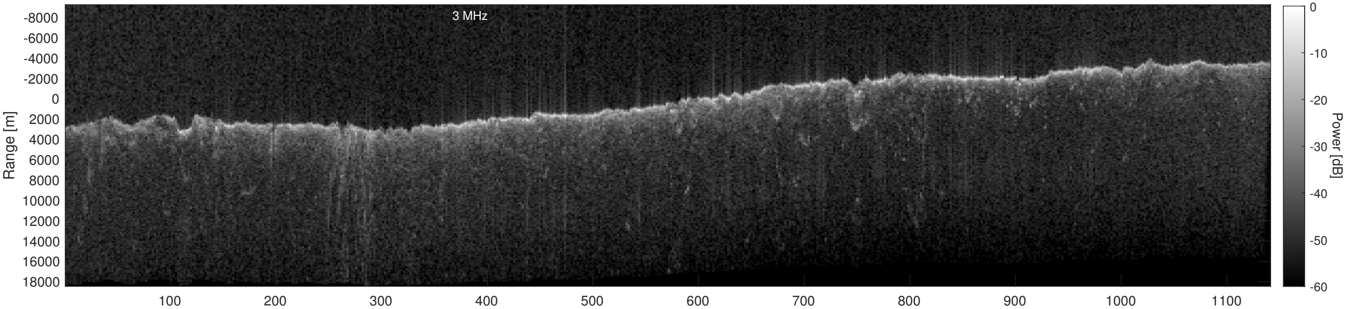
Orbit 17505, Depth-Corrected Cluttergram
