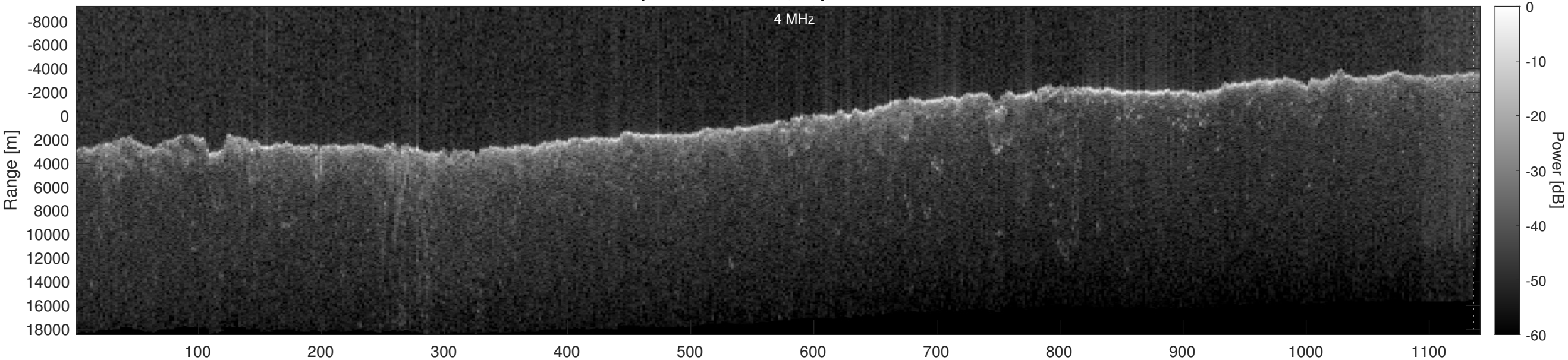
Orbit 17505, Optimized, Window, Depth-Corrected, Channel 2
