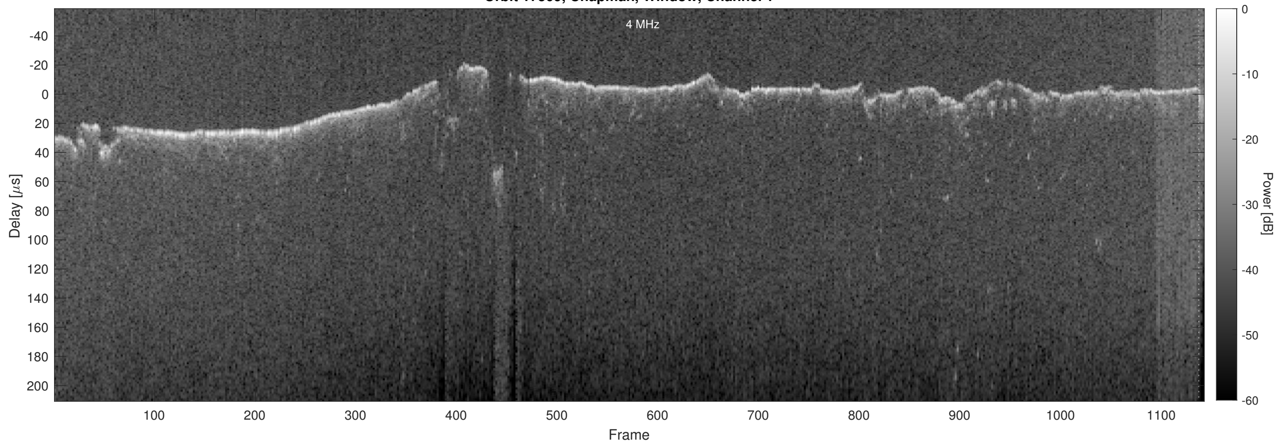
Orbit 17509, Chapman, Window, Channel 2
