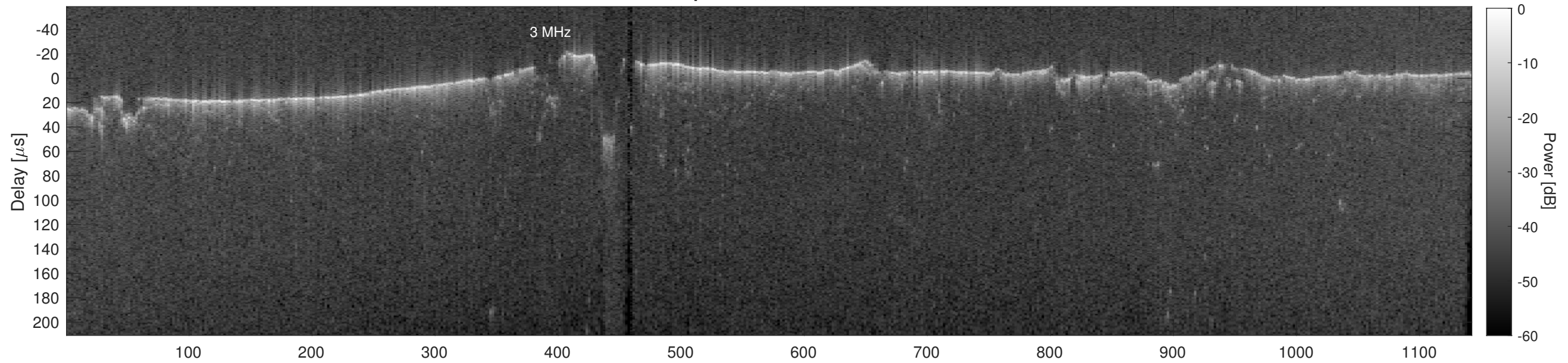
Orbit 17509, Cluttergram
