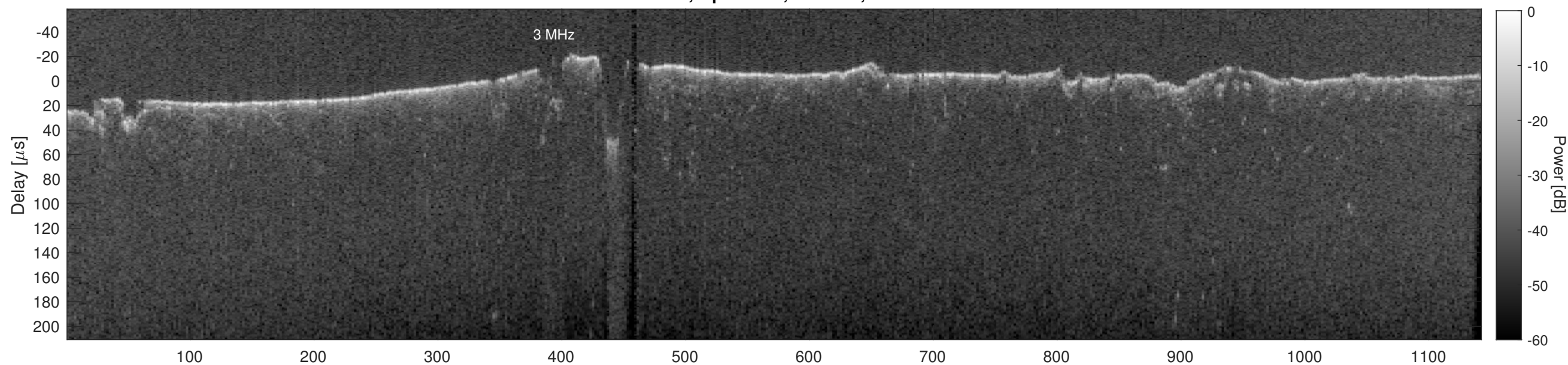
Orbit 17509, Cluttergram
