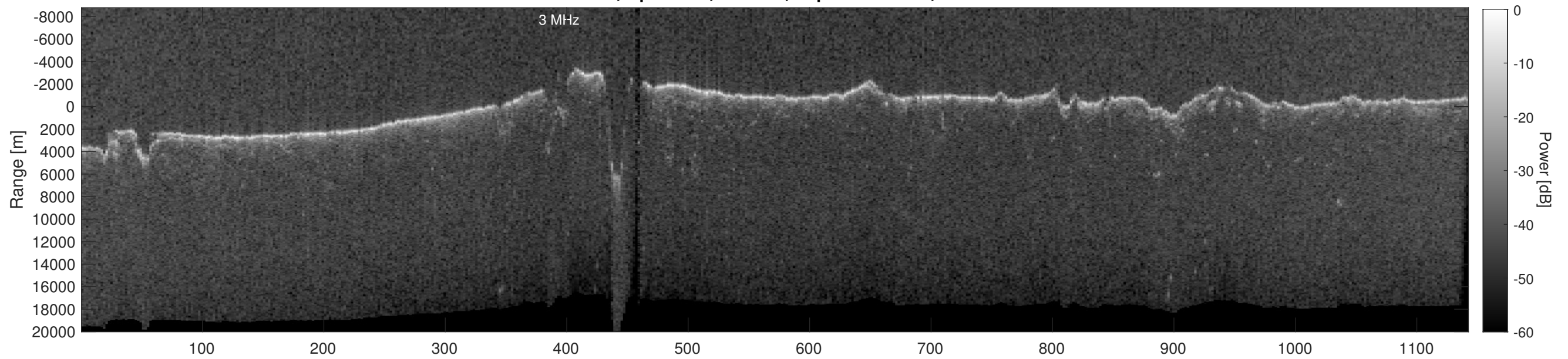
Orbit 17509, Depth-Corrected Cluttergram
