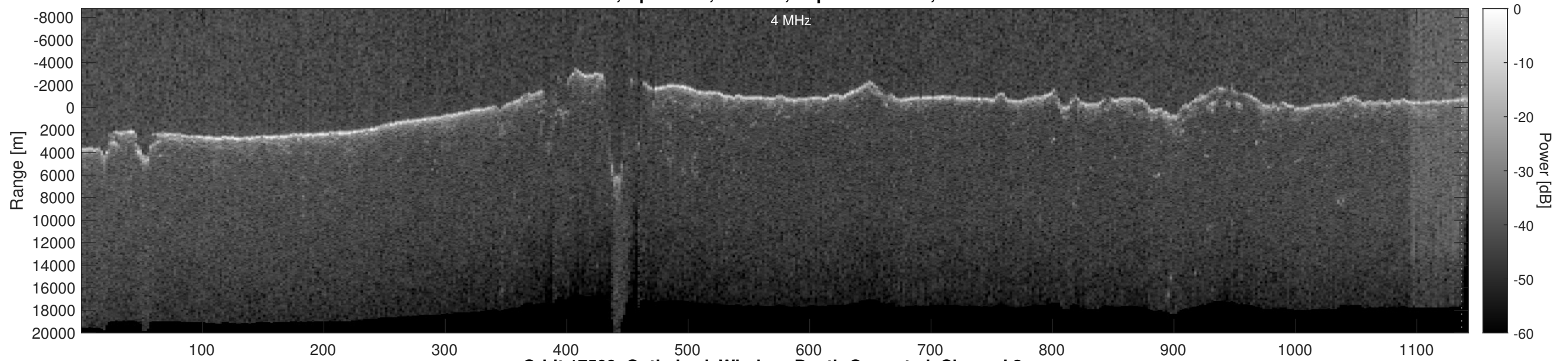
Orbit 17509, Optimized, Window, Depth-Corrected, Channel 2
