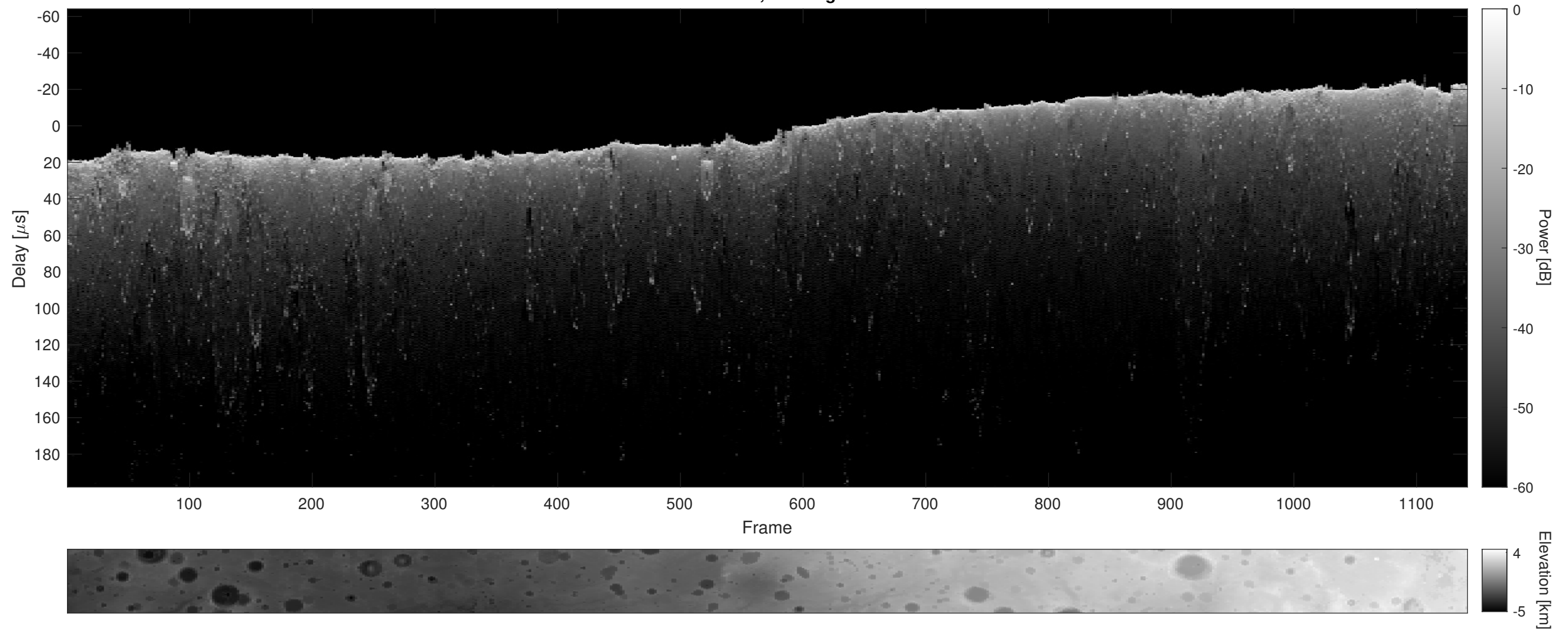
Orbit 17512, Cluttergram
