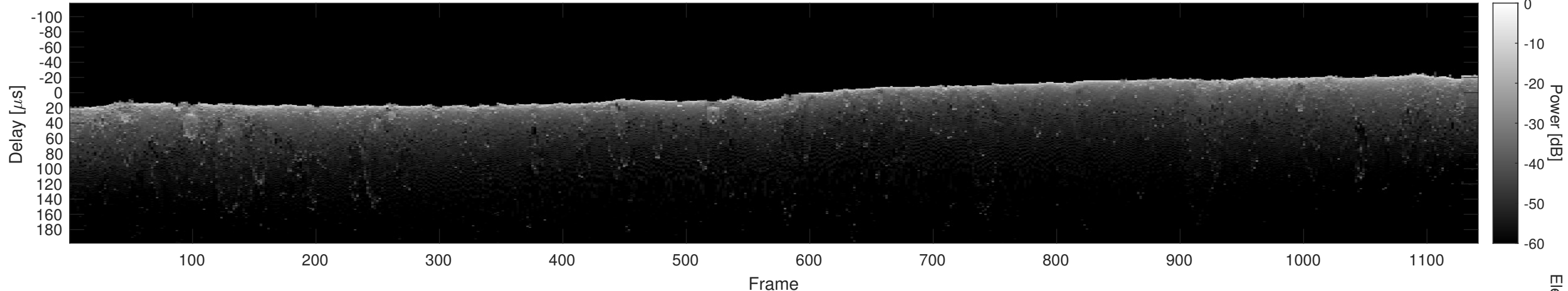
Orbit 17512, Cluttergram
