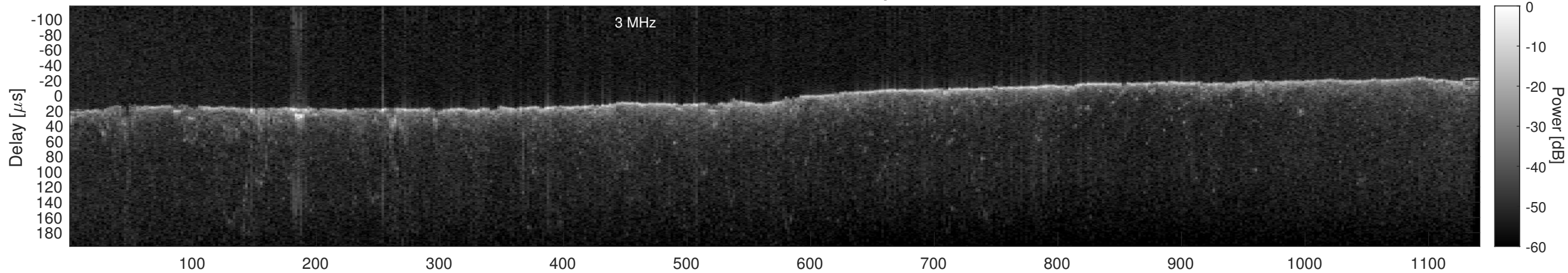
Orbit 17512, Cluttergram
