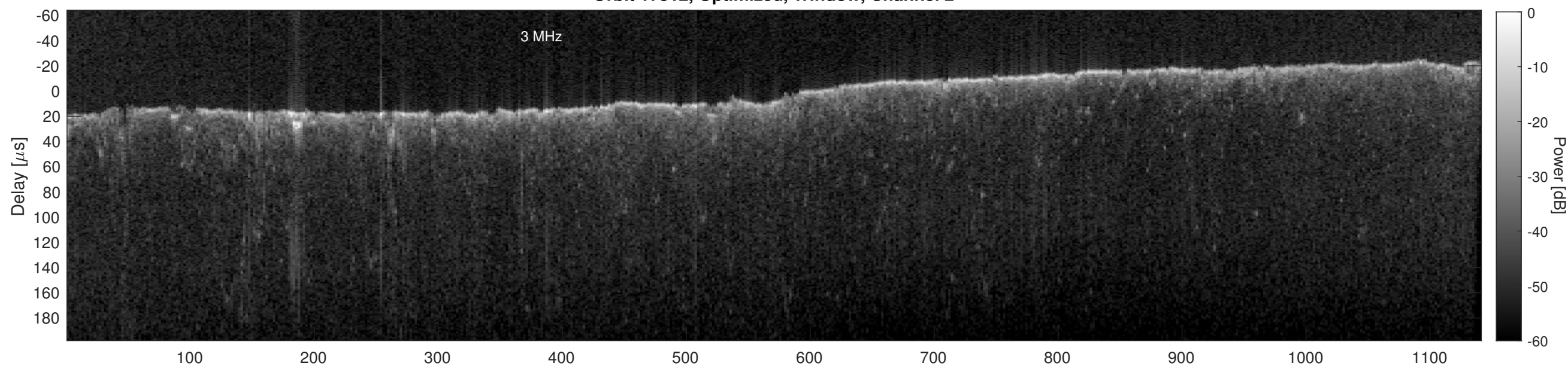
Orbit 17512, Cluttergram
