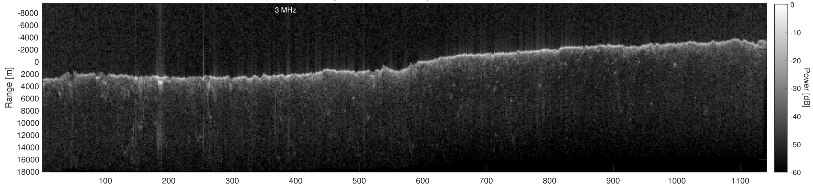
Orbit 17512, Depth-Corrected Cluttergram
