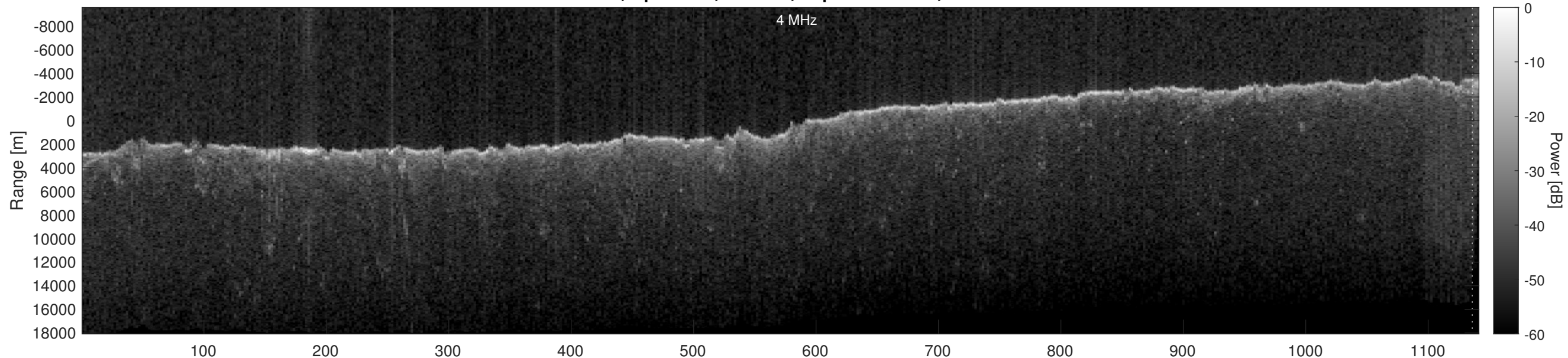
Orbit 17512, Optimized, Window, Depth-Corrected, Channel 2
