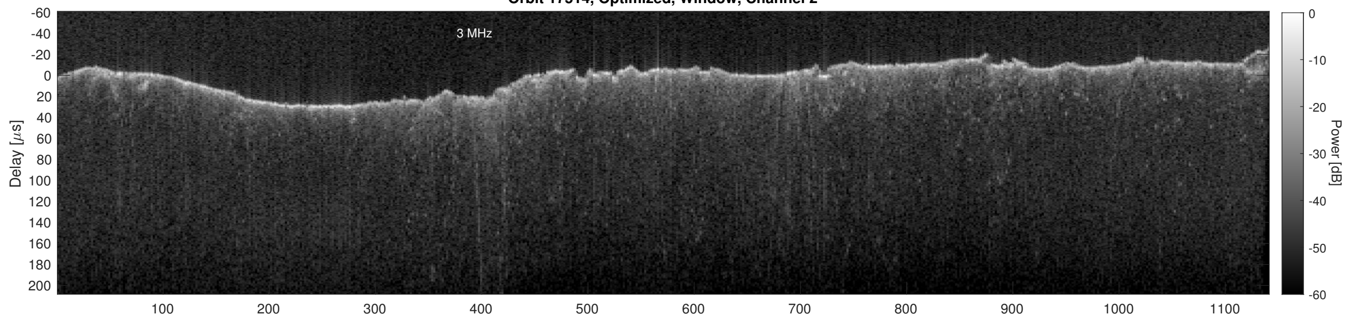
Orbit 17514, Cluttergram
