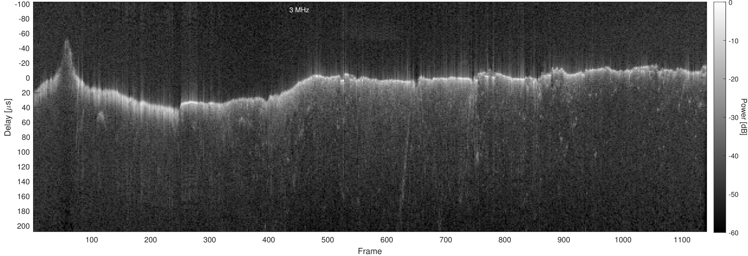
Orbit 17521, Chapman, No Window, Channel 2
