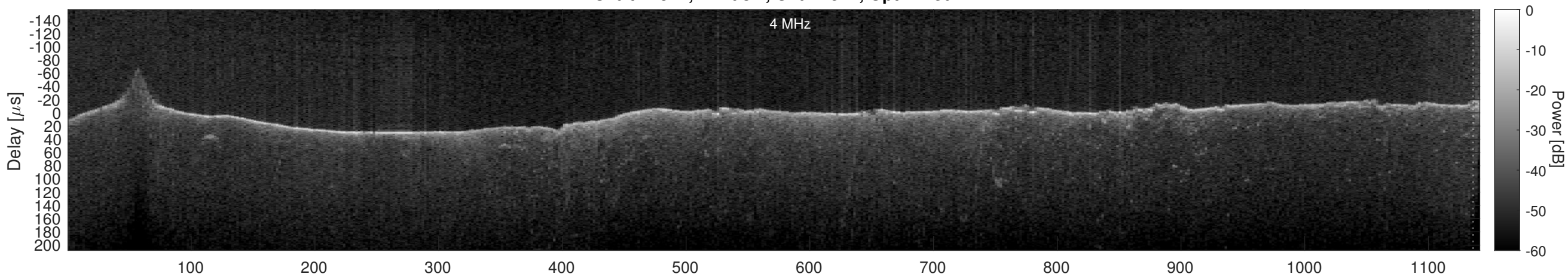
Orbit 17521, Cluttergram
