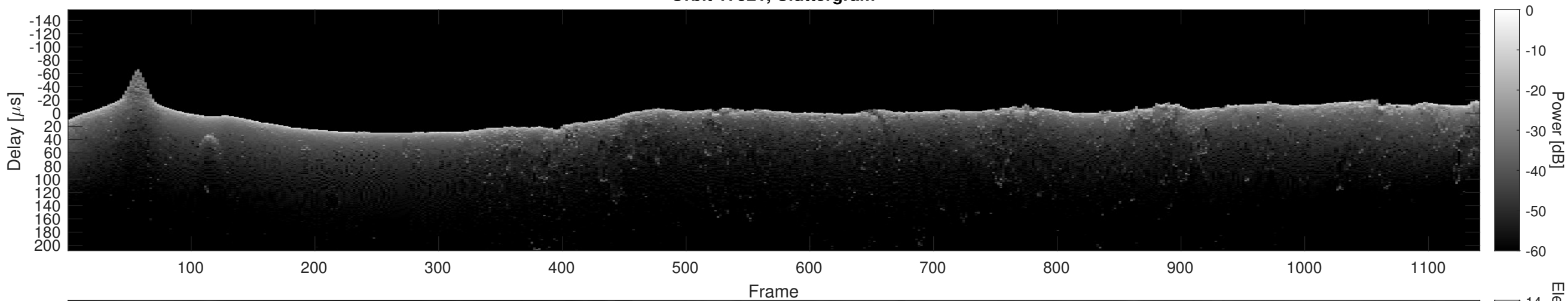
Orbit 17521, Cluttergram
