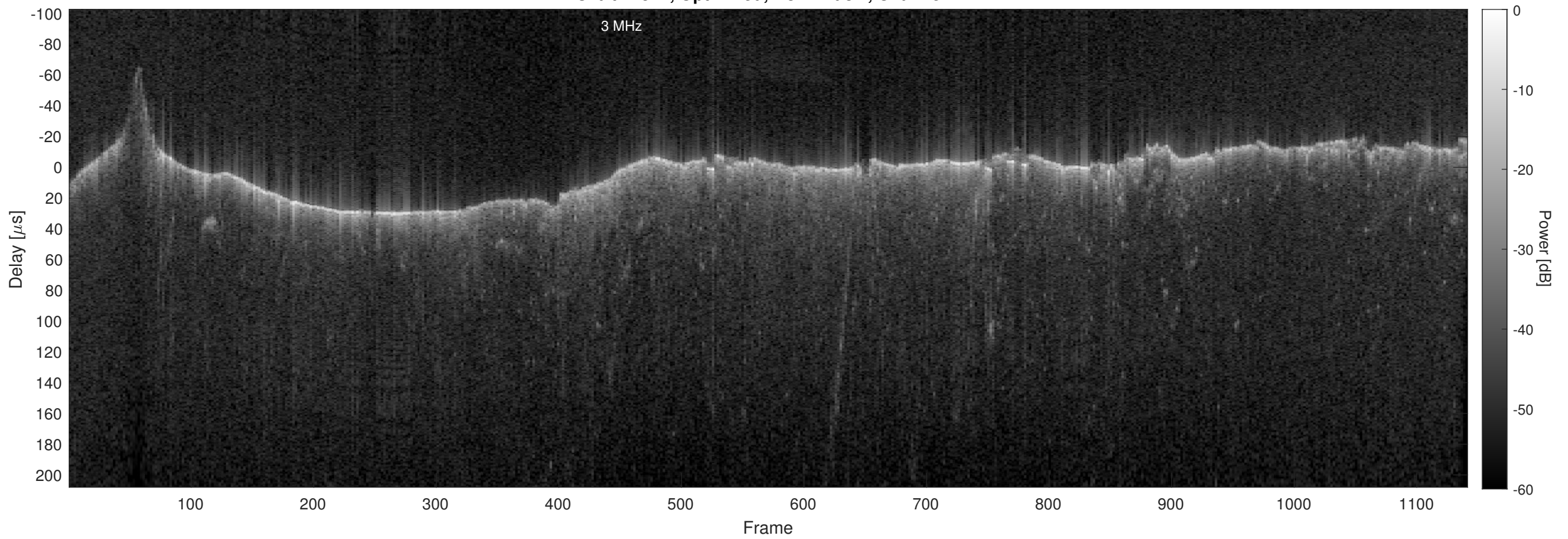
Orbit 17521, Optimized, No Window, Channel 2
