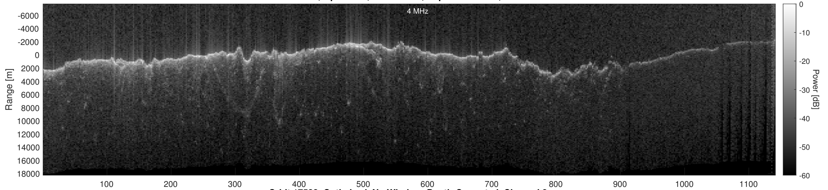
Orbit 17522, Optimized, No Window, Depth-Corrected, Channel 2
