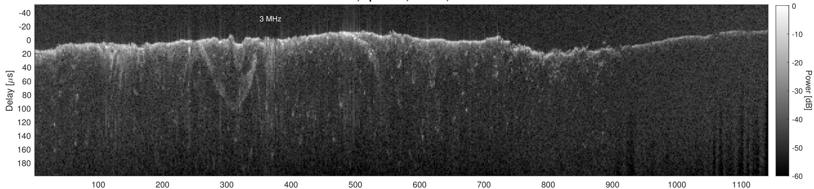
Orbit 17522, Cluttergram
