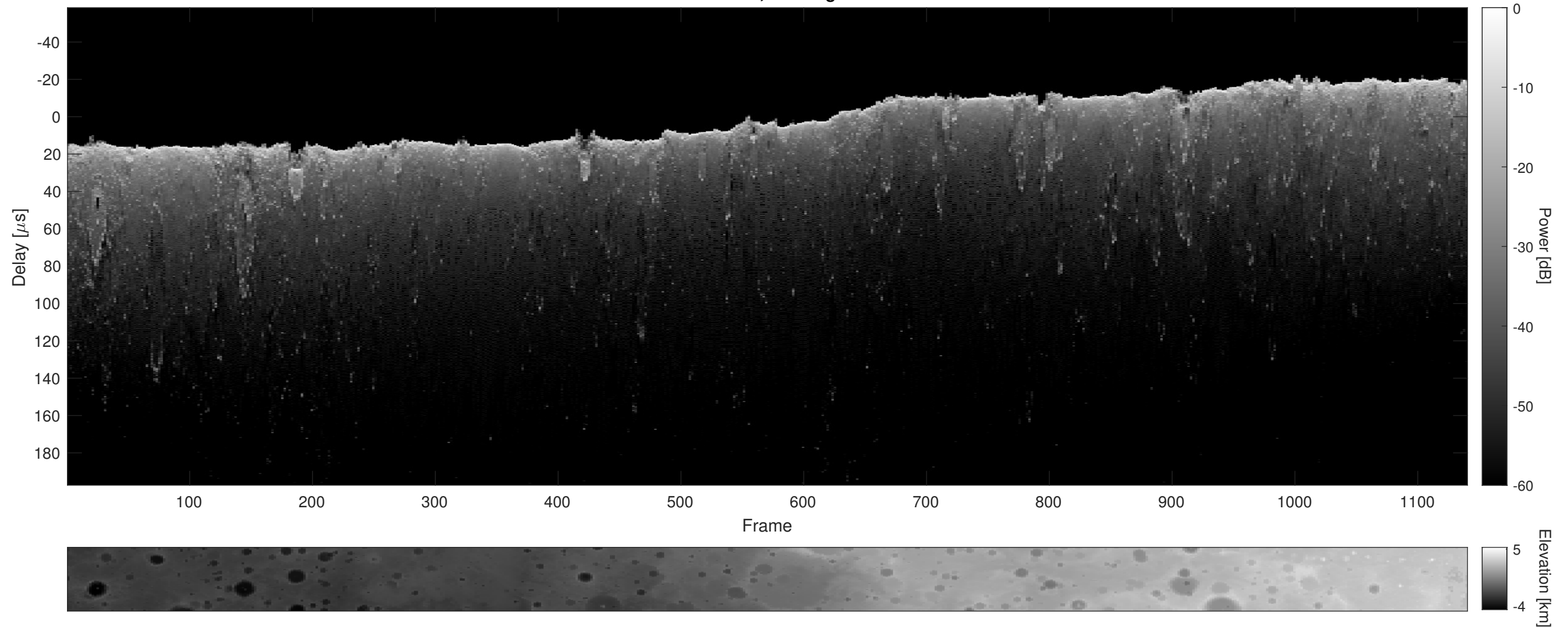
Orbit 17526, Cluttergram
