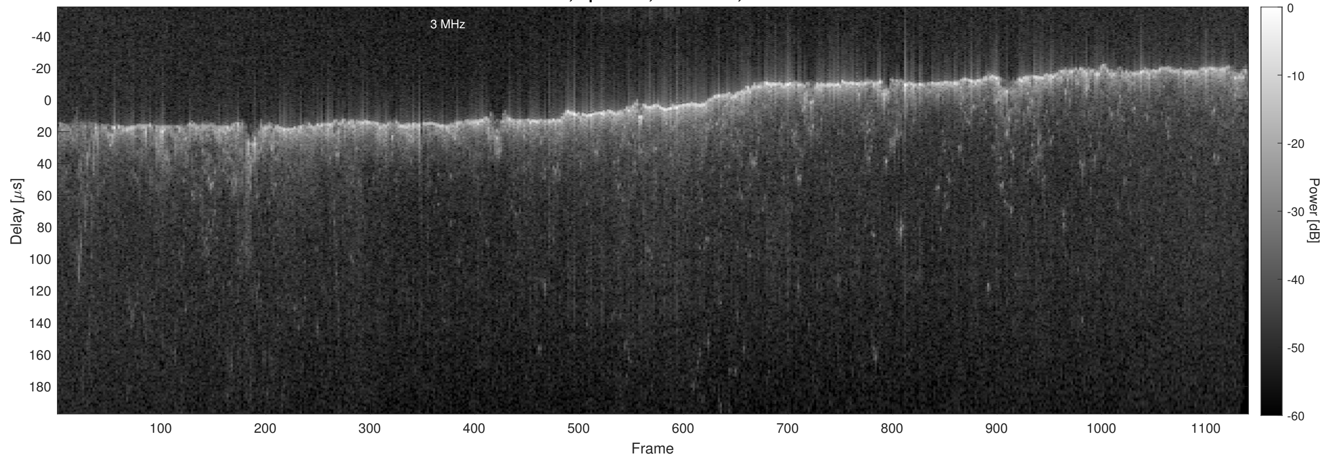
Orbit 17526, Optimized, No Window, Channel 2
