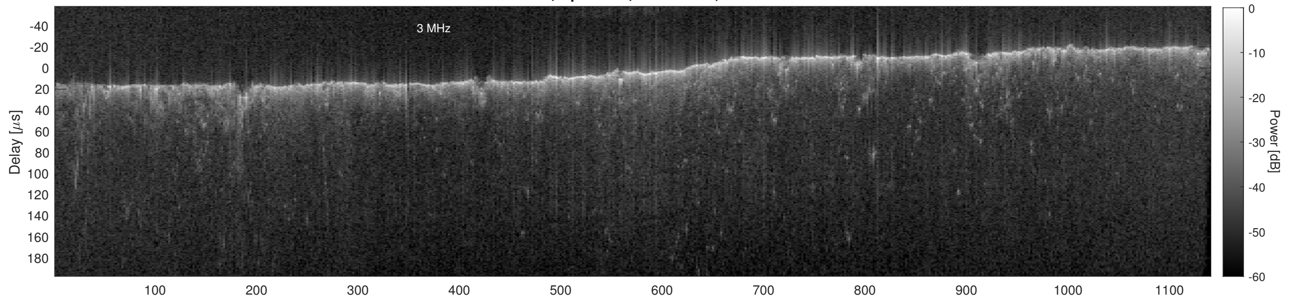
Orbit 17526, Cluttergram
